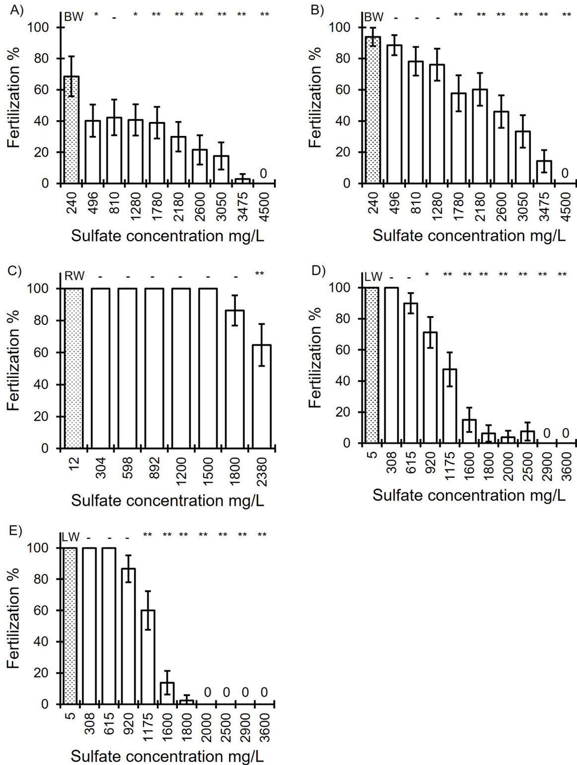
Fig. 1. Proportion of successfully fertilized eggs in brackish water vendace (A) (%), n = 51–104 eggs per treatment), brackish water whitefish (B) (%), n = 51–104 eggs per treatment), anadromous sea-migratory whitefish (C) (%), n = 50–51 eggs per treatment), freshwater vendace (D) (%), n = 55–80 eggs) and freshwater whitefish (E) (%), n = 55–80 eggs). Experiments done in different sulfate ( \text{SO}_4^{2-} ) treatments and in control treatments (BW = brackish water, RW = R. Kokemäenjoki water, LW = L. Konnevesi water) with background sulfate concentrations. The significance levels are above the bars (Kruskal-Wallis): – = P > 0.05 , * = P < 0.05 , ** = P < 0.01 . Vertical lines on bars represent the 95% confidence limits.
