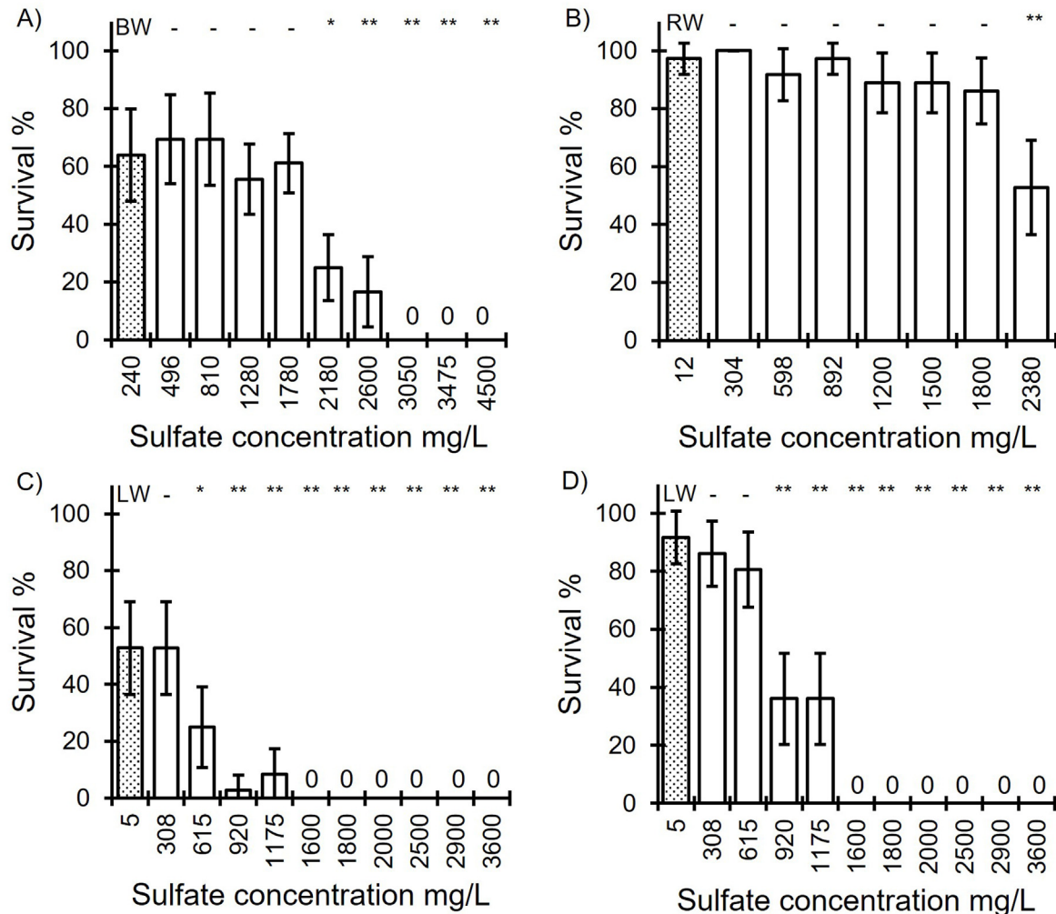
Fig. 2. Survival (%) of brackish water whitefish (A) (34 days from the fertilization, n=36 ), anadromous sea-migratory whitefish (B) (25 days from the fertilization, n=36 ), freshwater vendace (C) (34 days from the fertilization, n=36 ) and freshwater whitefish (D) (34 days from the fertilization, n=36 ) in the early embryonic phase from fertilization to eyed stage in different sulfate ( \text{SO}_4^{2-} ) concentrations with control treatments (BW = brackish water, RW = R. Kokemäenjoki water, LW = L. Konnevesi water) and their background \text{SO}_4^{2-} concentrations. The significance levels are above the bars (Kruskal-Wallis): - = P > 0.05 , * = P < 0.05 , ** = P < 0.01 . Vertical lines on bars represent the 95% confidence limits.
