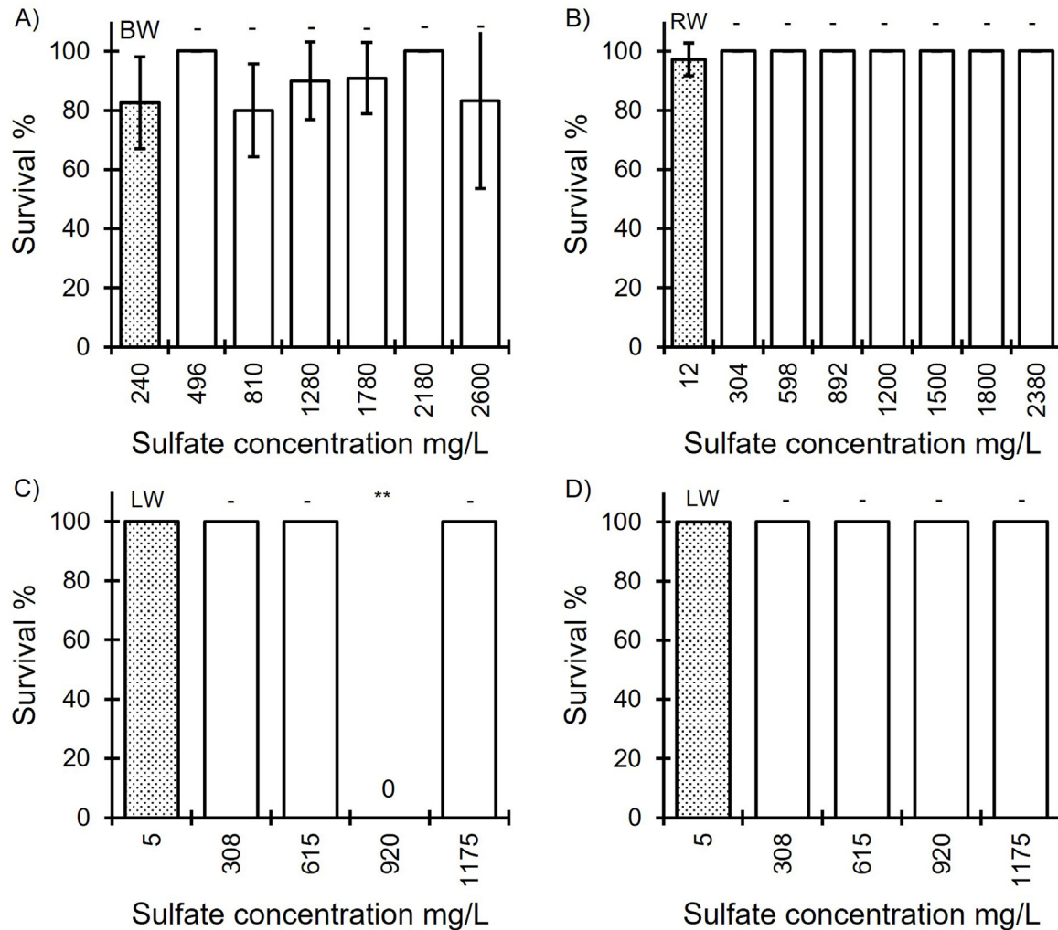
Fig. 3. Survival (%) of brackish water whitefish (A) (169 days from the end of early embryonic period, n=36 ), anadromous sea-migratory whitefish (B) (140 days from the end of early embryonic period, n=36 ), freshwater vendace (C) (175 days from the end of early embryonic period, n=36 ) and freshwater whitefish (D) (186 days from the end of early embryonic period, n=36 ) during the late embryonic phase, hatching and larval period in different sulfate ( \text{SO}_4^{2-} ) concentrations with control treatments (BW = brackish water, RW = R. Kokemäenjoki water, LW = L. Konnevesi water) and their background \text{SO}_4^{2-} concentrations. The significance levels are above the bars (Kruskal-Wallis): – = P > 0.05 , * = P < 0.05 , ** = P < 0.01 . Vertical lines on bars represent the 95% confidence limits.
