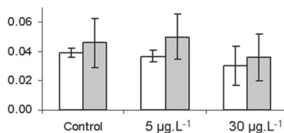
Fig. 2. Biofilm biomass ( \pm S.E.) on glass slides after 14 days of experiment, expressed as ash-free dry mass (AFDM, white bars, \text{mg.cm}^{-2} ) and as chlorophyll- a (grey bars, \text{mg.dm}^{-2} ).
