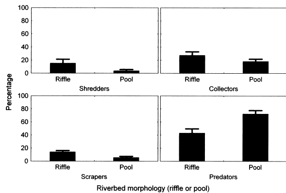
Fig. 4. Response of functional attributes of caddisflies (shredders, collectors, scrapers and predators) to riverbed morphology.
