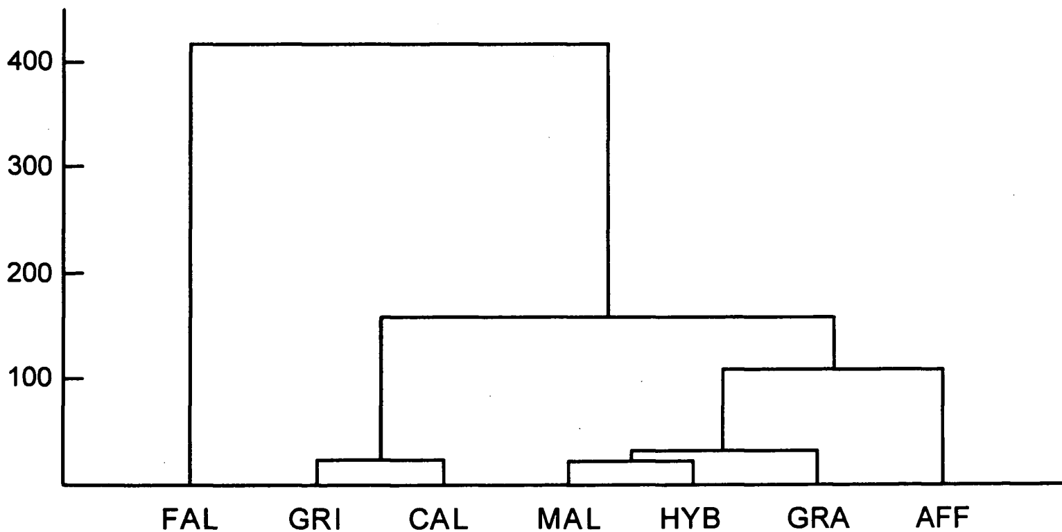
Fig. 22. Unweighted pair group average dendrogram based on Mahalanobis distance between pairs of species (without N_HFF ; cophenetic correlation=0.873).
