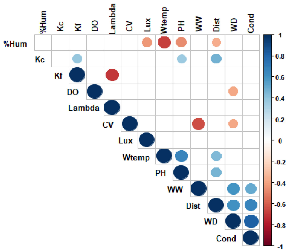
Fig. 5. Pearson correlations between decomposition metrics ( K_c , K_f , \lambda_F ) and environmental factors. The values represent the correlation coefficients. The coloured squares represent the significant coefficients (red or blue, P -value < 0.05 ) according to the scale of the value indicated on the right of the correlogram.
